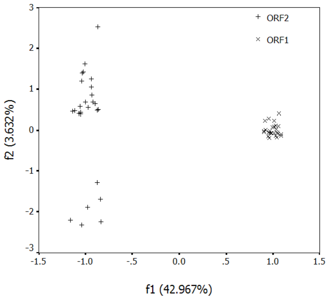
The first axis ( f_1 ) accounts for 42.967% of the total variation, and the second axis ( f_2 ) accounts for 3.632% of the total variation.
