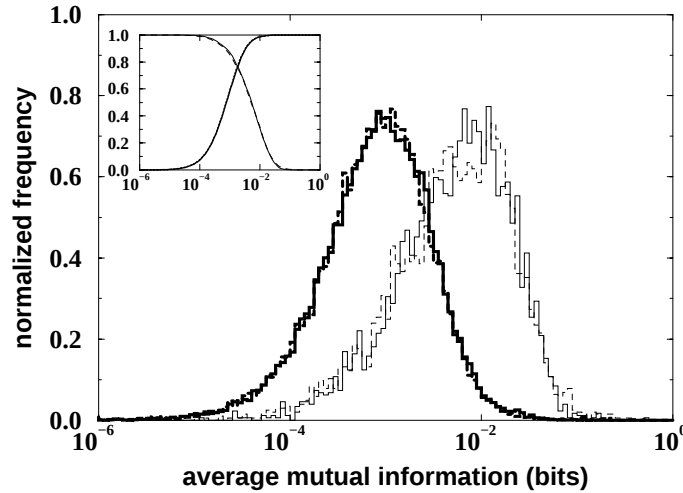
Figure 2: AMI distributions of data sets hung108a (solid lines) and hung108b (dashed lines) of Fickett and Tung 1 for coding DNA (thin lines) and noncoding DNA (thick lines). In both data sets the AMI distribution of noncoding DNA is centered at significantly smaller values than the AMI distribution of coding DNA. The cumulative distribution functions of the AMI presented in the inset show that the AMI allows a discrimination of coding and noncoding DNA with an accuracy of approximately 76%.
